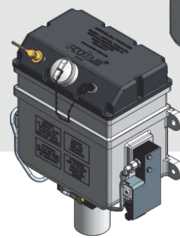
Pneumatic pump Flui 1 - 13,0 kg with directional valve
