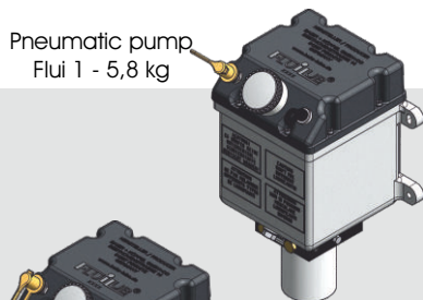
Pneumatic pump Flui 1 - 5,8 kg with mixing distributor
