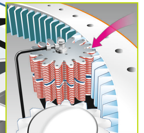
The BEKAWIND lubricating pinion supplies only the contact zone
